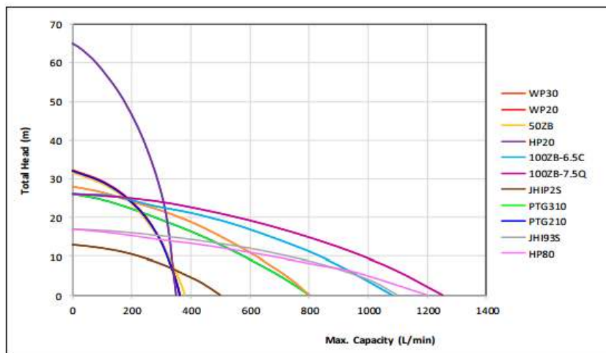
HP20 2" High Pressure Pump
